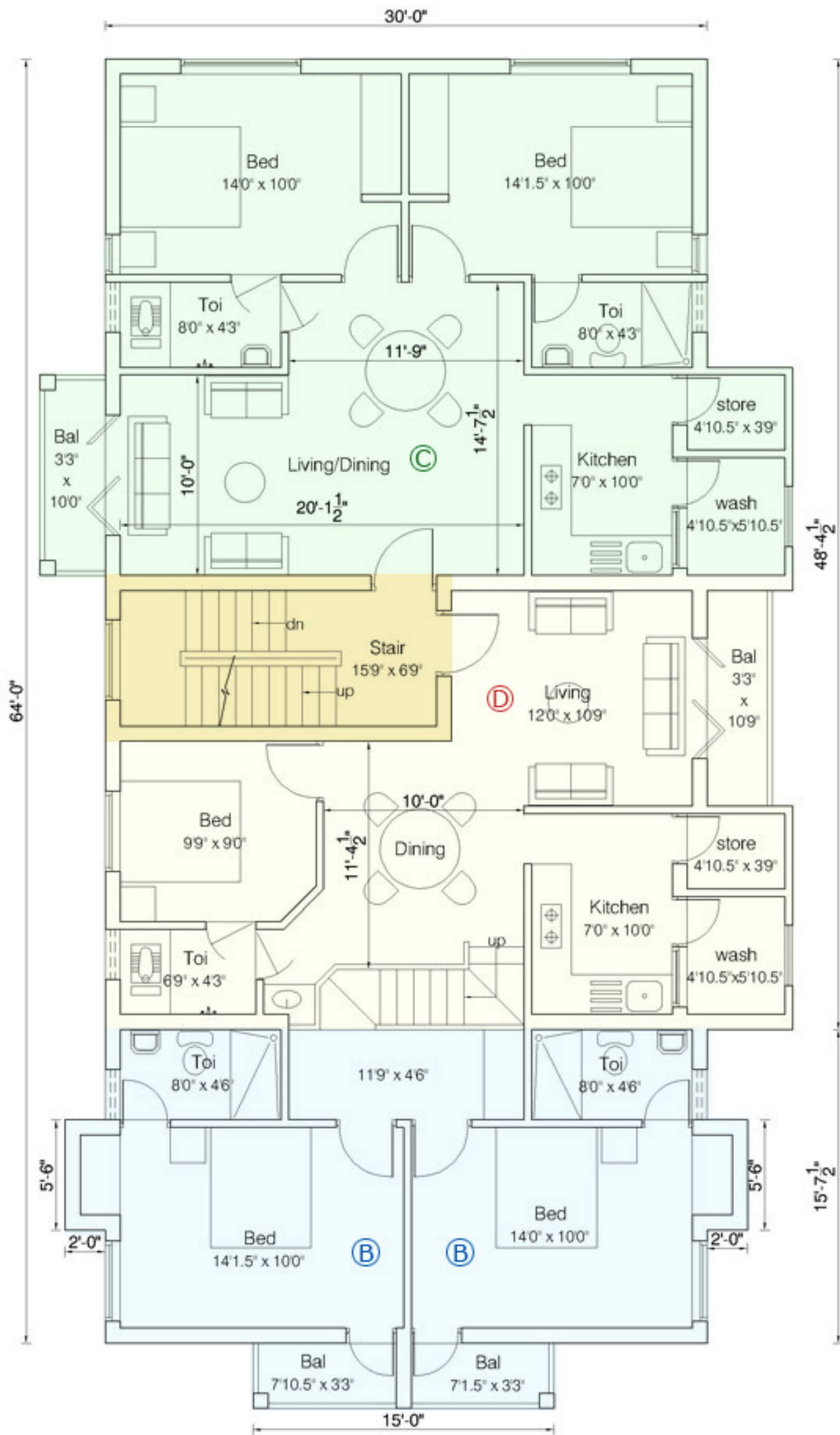
FIRST FLOOR PLAN Block - 1
