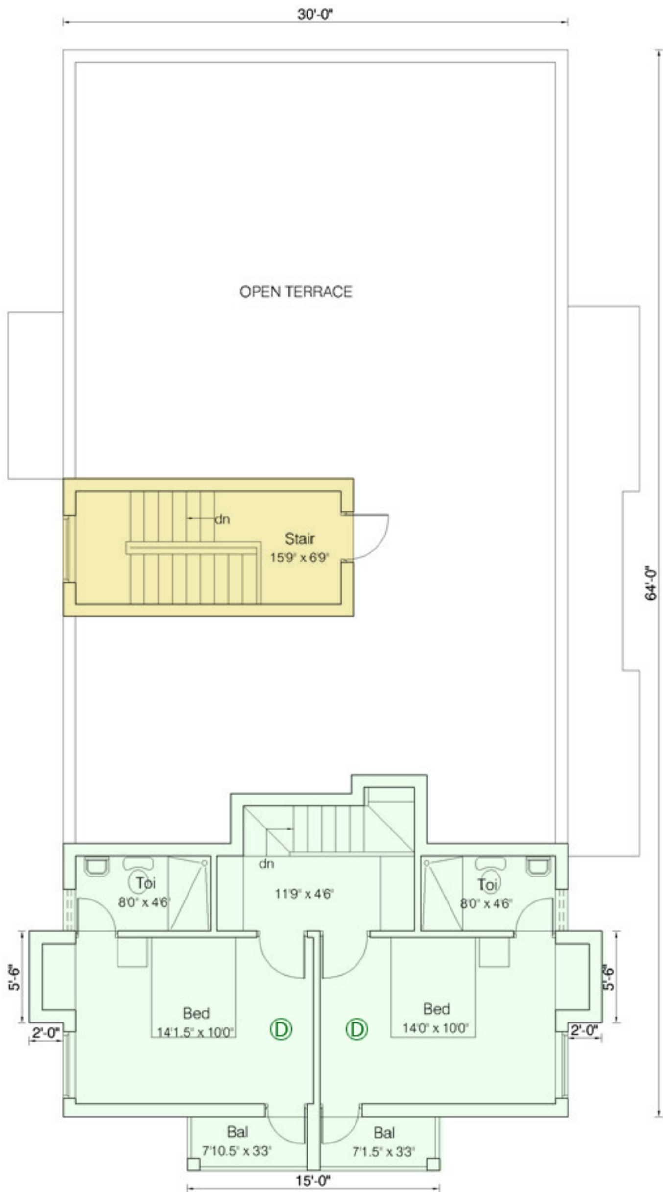
SECOND FLOOR PLAN Block - 1
