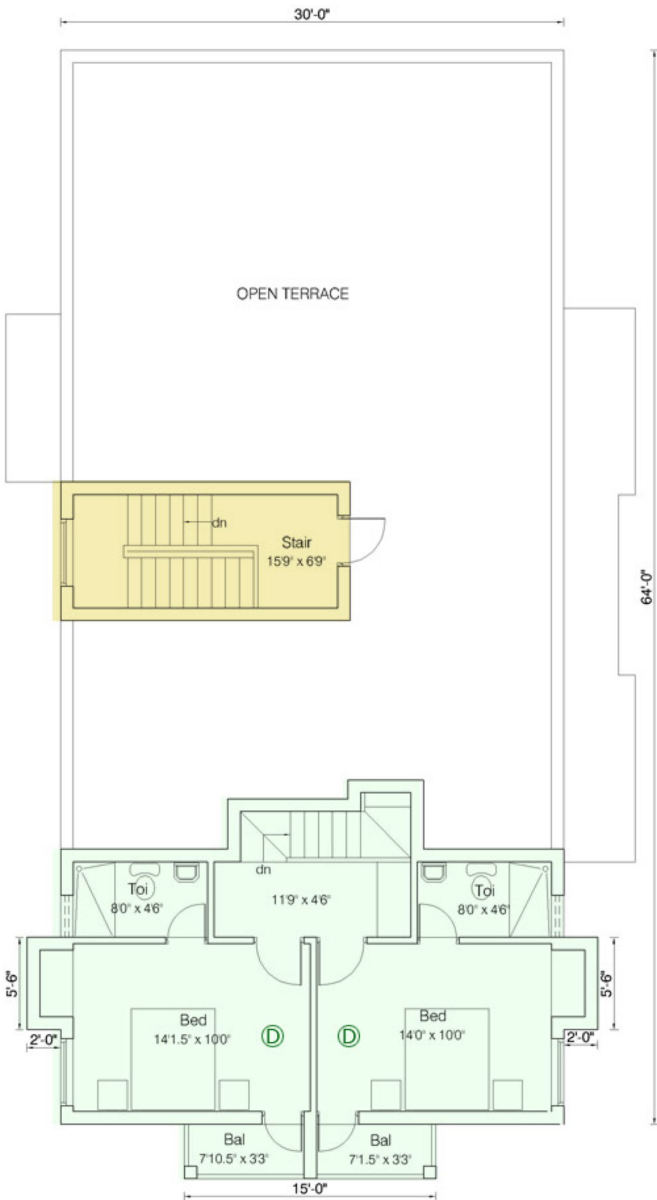
SECOND FLOOR PLAN Block - 2
