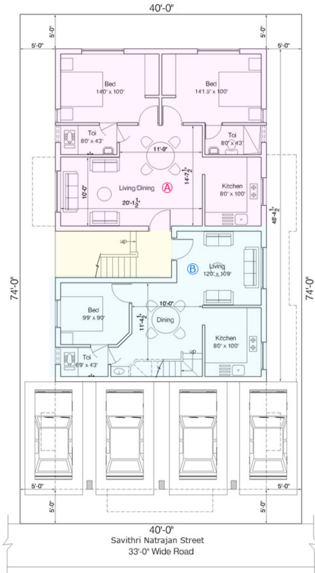
SITE/GROUND FLOOR PLAN
